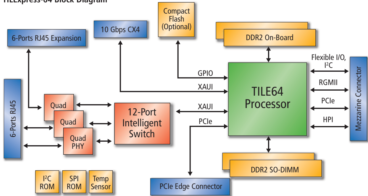
TILExpress-64 Block Diagram
